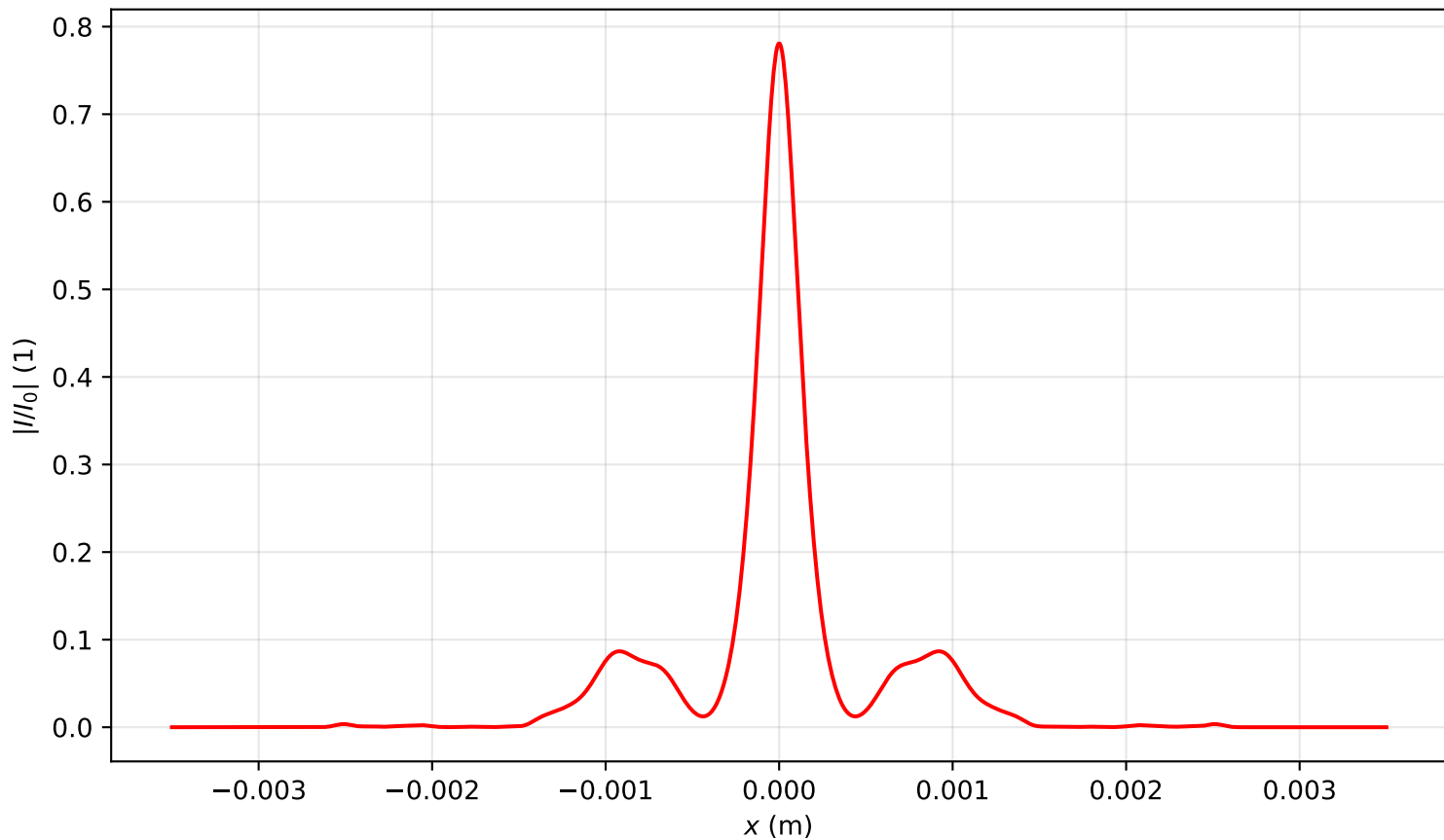
Intensity profile I(x, y = 0, z = 1.911)/I_0 , P_{in}=8.5P_{cr} , artificial time
